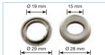
303-501 Asola tornichetto in nylon (2pz) col. bianco/nero Nylon grommer for turnbutton (2pcs) col. white/black
